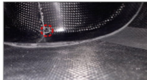
The front trumpet should have a 8mm drain hole at the bottom. Invisible for the eye, could be found by touch or with a mirror.
