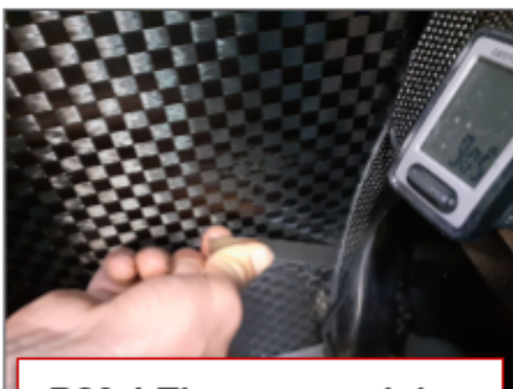
B20.1 The proper gluing can be tested with a cutter blade
